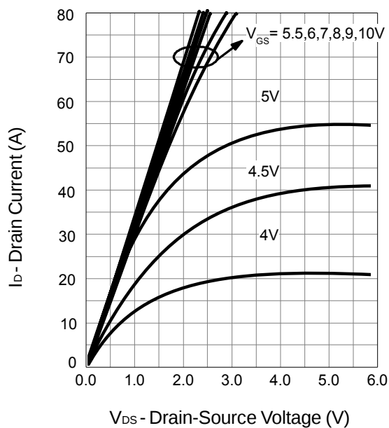
Output Characteristics
